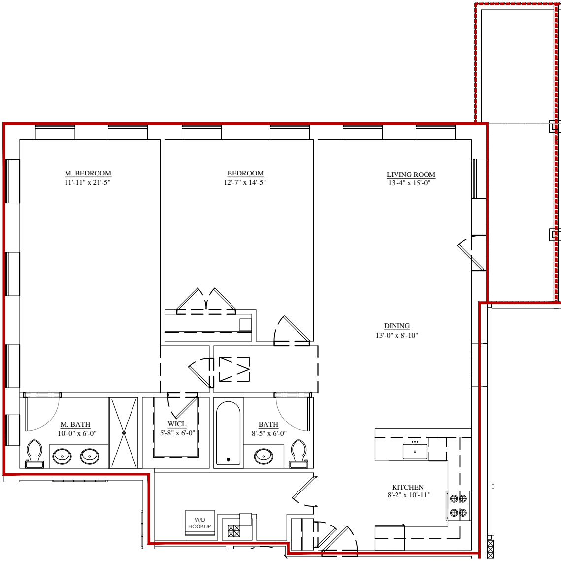
SECOND FLOOR PLAN_APT 205
