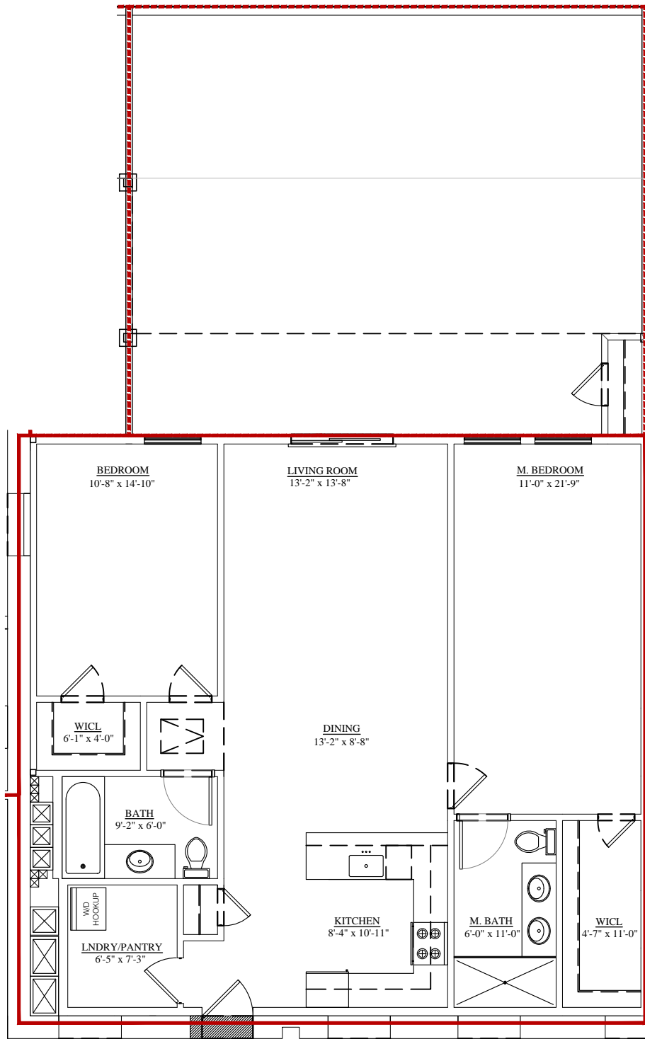
SECOND FLOOR PLAN_APT 206
